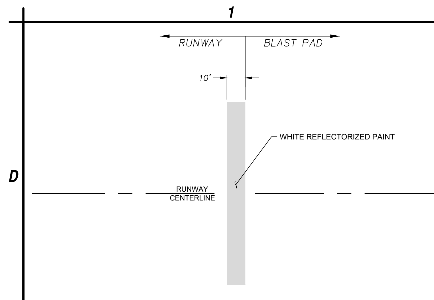
D1 THRESHOLD BAR MARKING NOT TO SCALE
