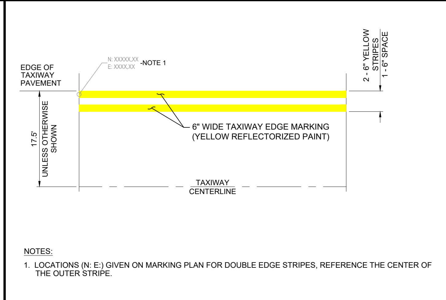
B4 CONTINUOUS TAXIWAY EDGE MARKING DETAIL NOT TO SCALE
