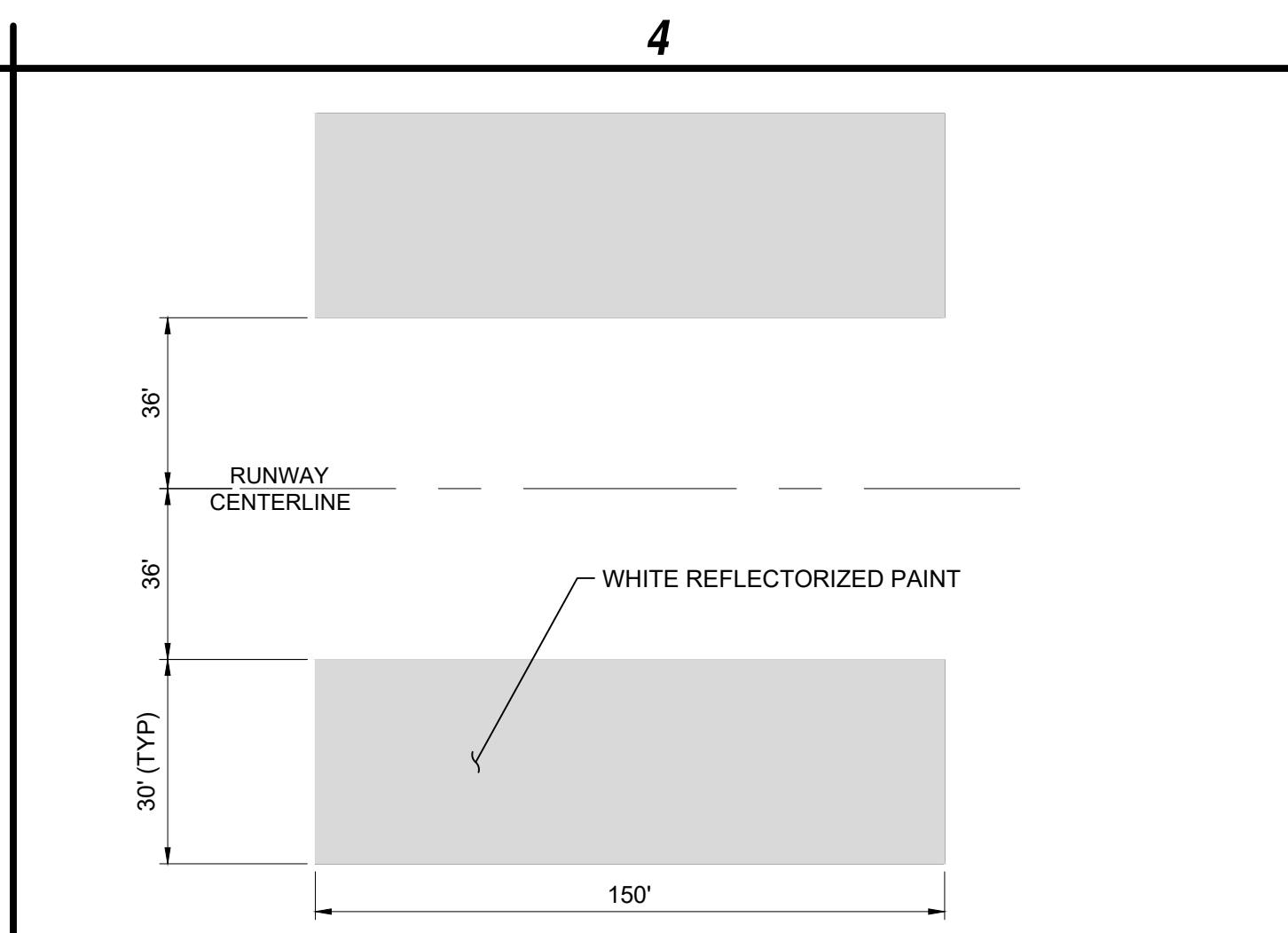
D4 AIMING POINT MARKINGS NOT TO SCALE
