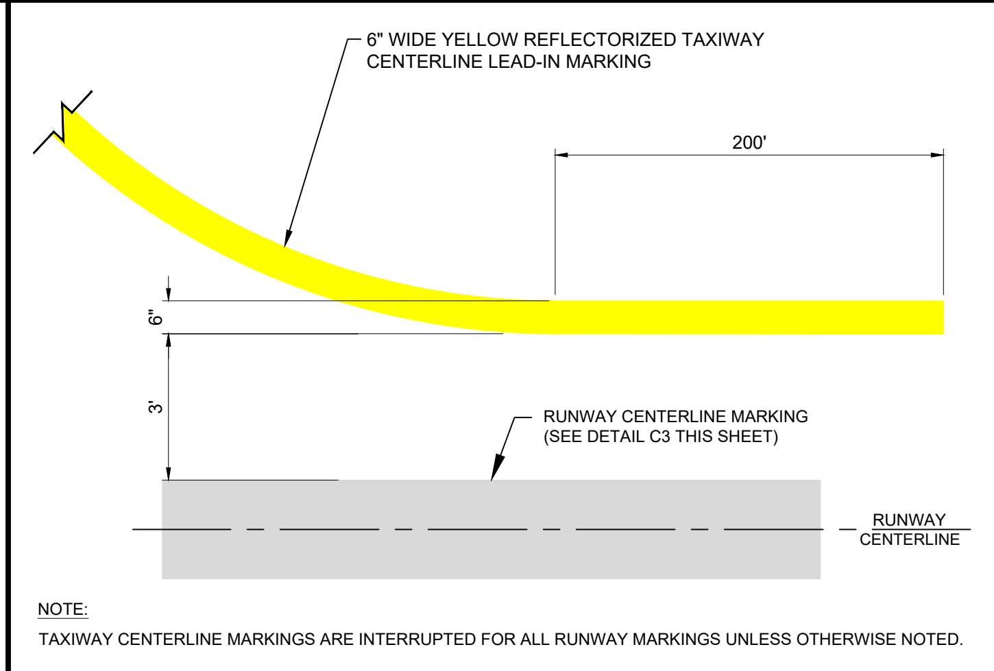
C2 TAXIWAY CENTERLINE LEAD-IN MARKING SCALE EXAGGERATED TO SHOW DIMENSIONS
