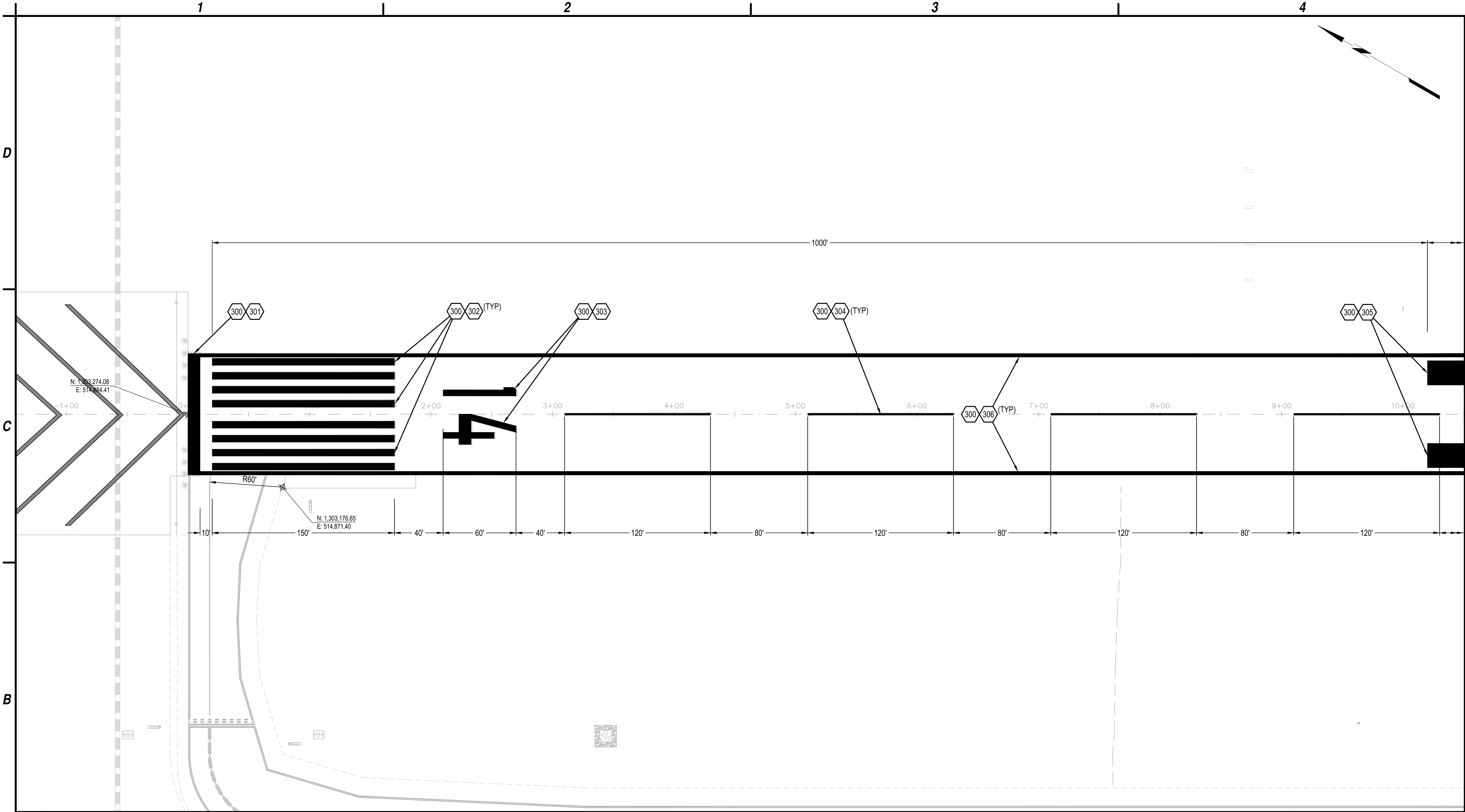
B1 IMPROVEMENT PLAN SCALE: 1"=50'
