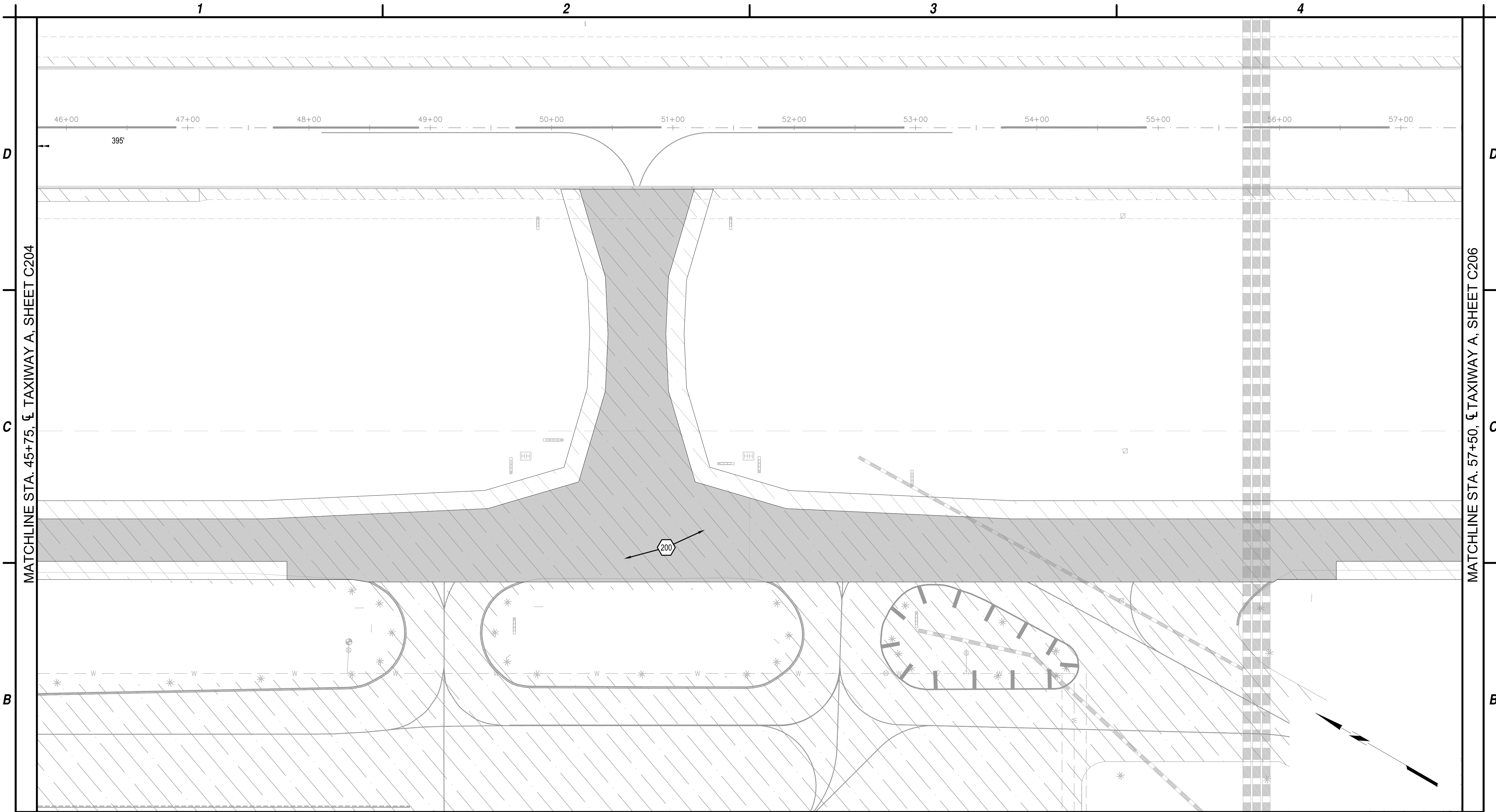
B1 IMPROVEMENT PLAN SCALE: 1"=50'
