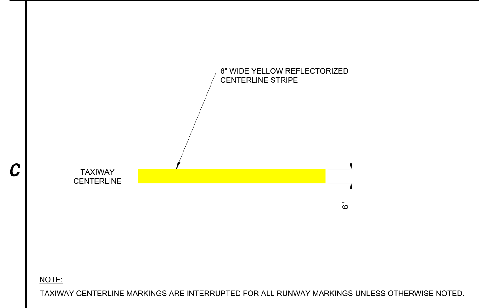
C1 TAXIWAY CENTERLINE MARKING DETAIL NOT TO SCALE
