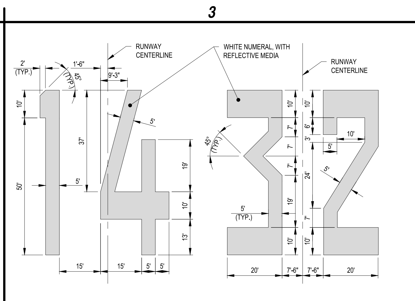
D3 RUNWAY DESIGNATOR MARKINGS NOT TO SCALE
