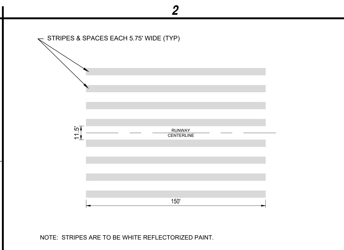
D2 THRESHOLD MARKING NOT TO SCALE
