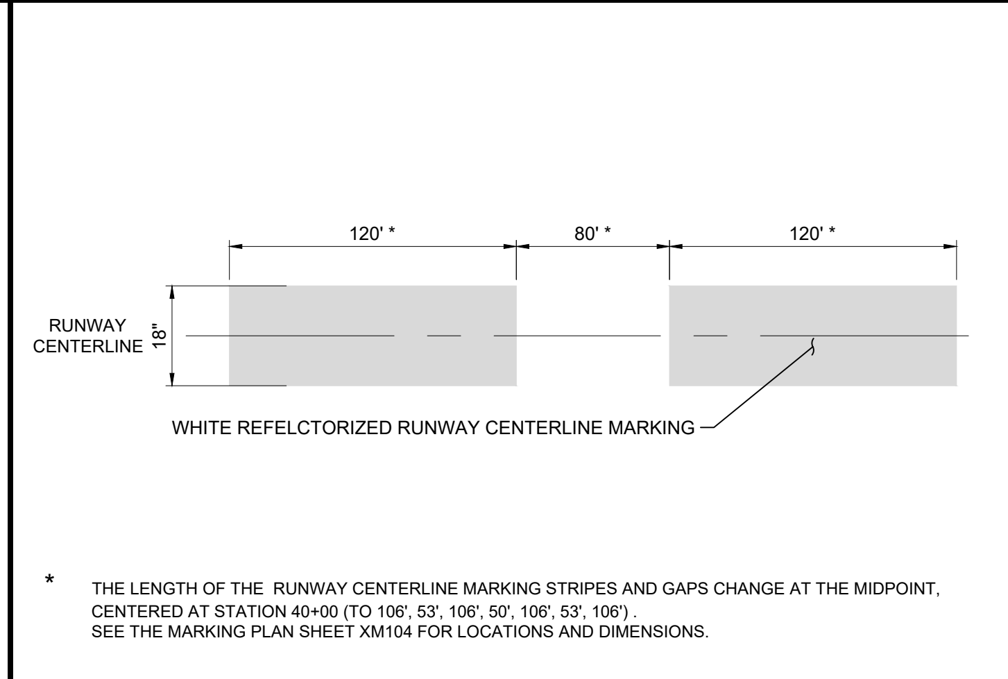
C3 RUNWAY CENTERLINE MARKINGS NOT TO SCALE
