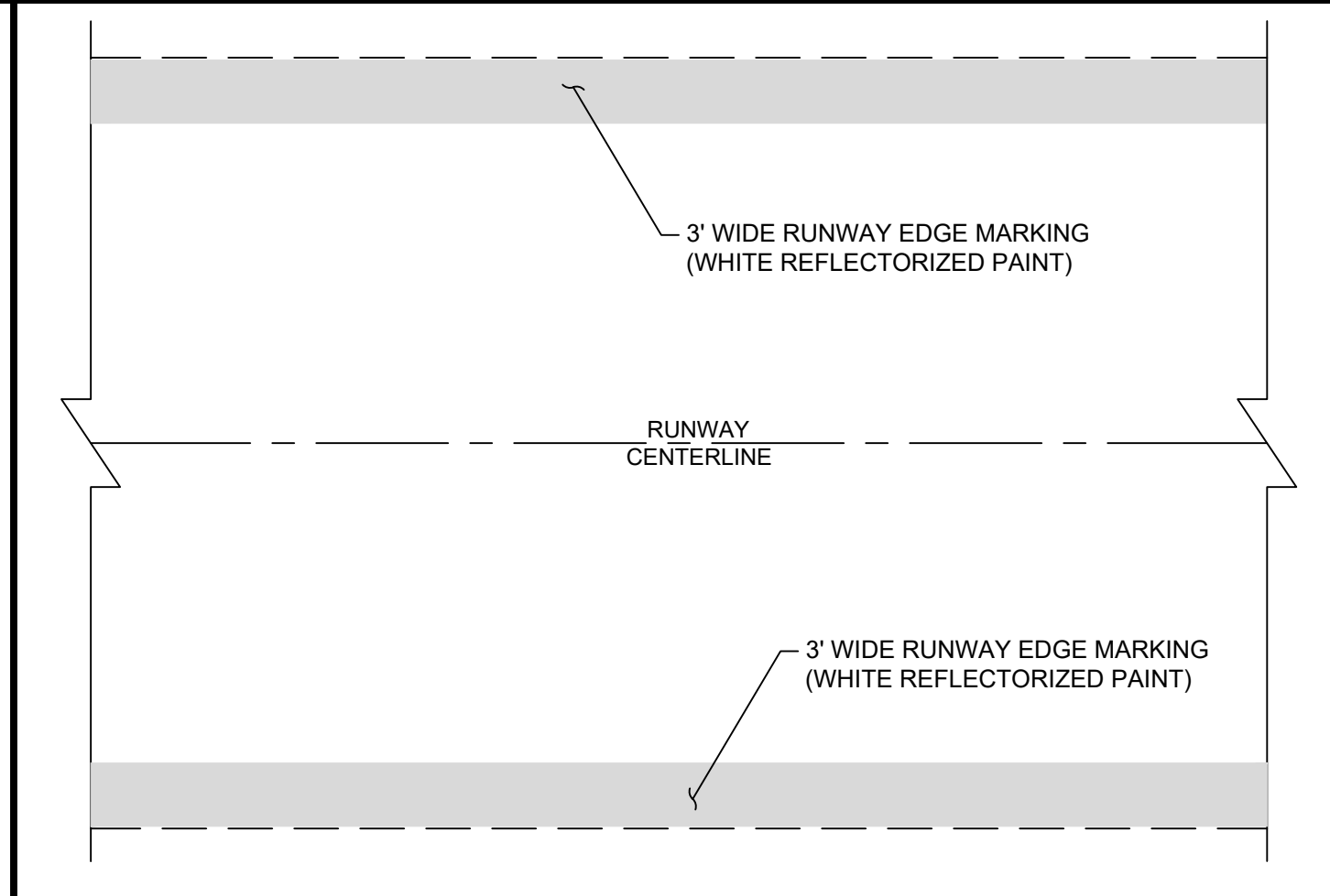
C4 RUNWAY EDGE MARKINGS NOT TO SCALE
