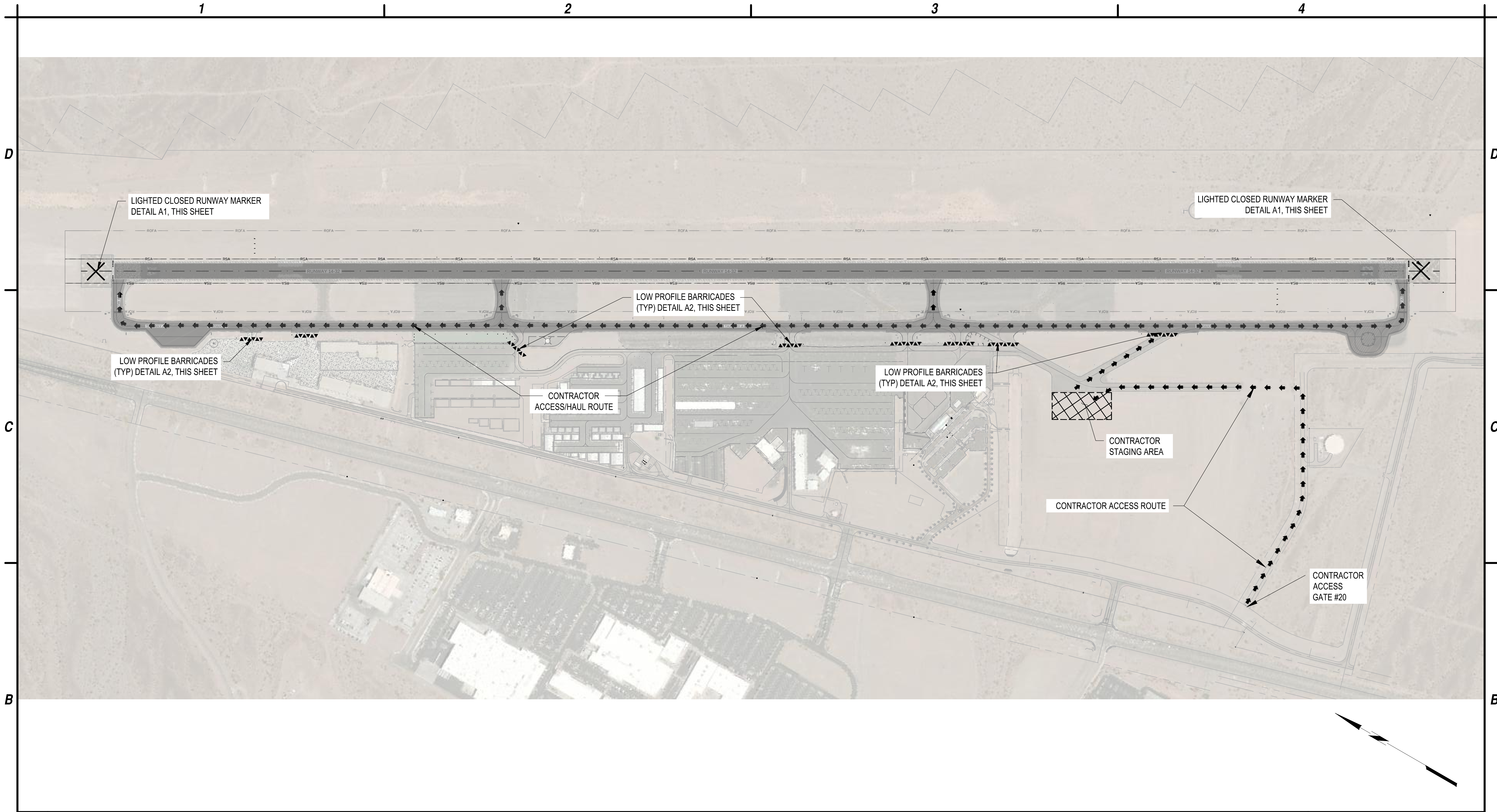
B1 CONSTRUCTION SAFETY AND PHASING PLAN SCALE: 1:300'
