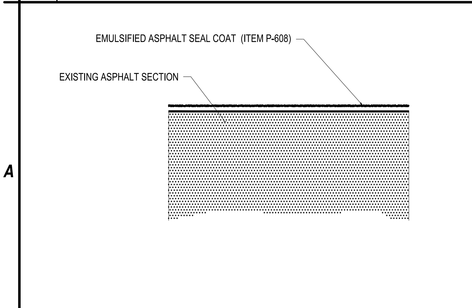
A1 ASPHALT EMULSION SEAL DETAIL NOT TO SCALE
