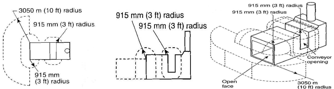
Figure 516.3(B)(2) Class I, Division 2, Class I, Zone 2, or Class II, Division 2 Locations Adjacent to a Closed Top, Open Face, or Open Front Spray Booth or Room. [NFPA 33:Figures 6.5.2(a) and 6.5.2(b)]
